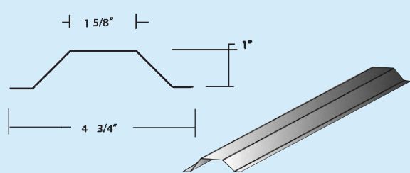
1" Sub-Girt
