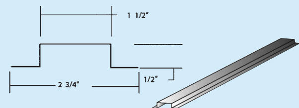
1/2" Sub-Girt
