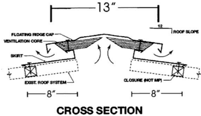
Continuous Ridge Vent
