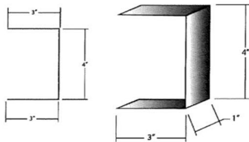
Downspout Strap
