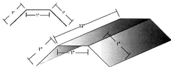
Gutter Strap (PBR-Panel)
