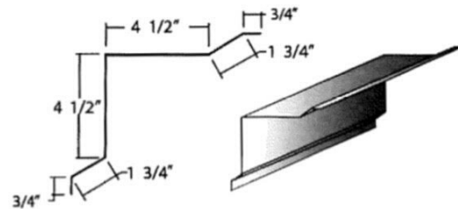
Inside Corner Trim (PBR-Panel)
