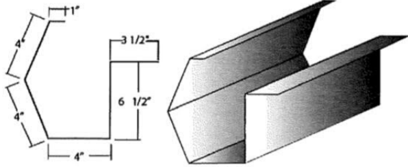
Sculptured Eave Gutter (PBR-Panel)
