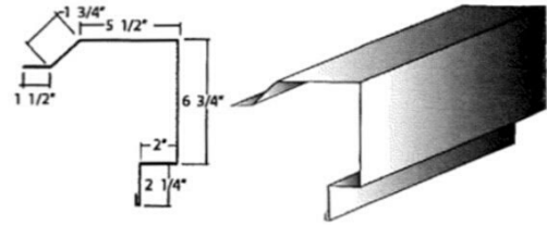
Box Rake (PBR-Panel)
