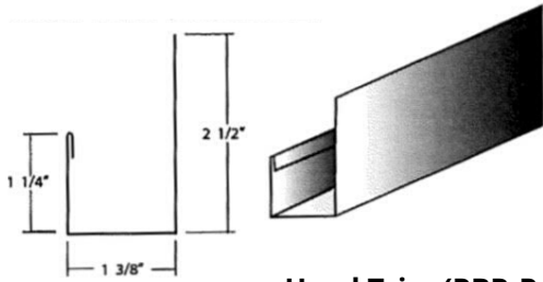
Head Trim (PBR-Panel)
