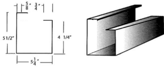
Box Hang-On Gutter
