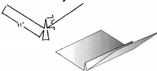
Standard Valley
