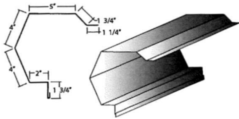
Sculptured Rake (PBR-Panel)
