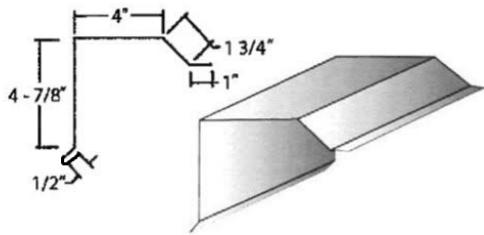
Rake Trim
