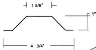
1 " Sub-Girt
