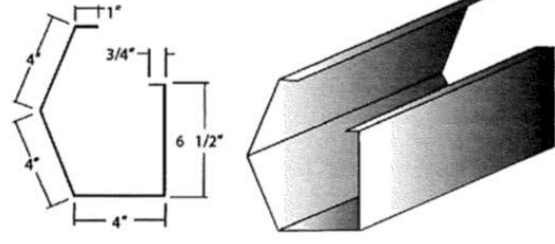
Sculptured Hang-On Gutter (PBR-Panel)
