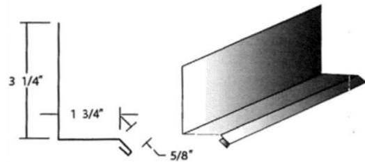
Base Trim
