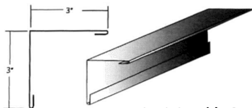
3 x 3 Outside Angle
