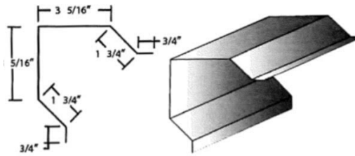
Outside Corner Trim (PBR-Panel)
