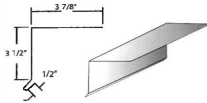
Eave Trim
