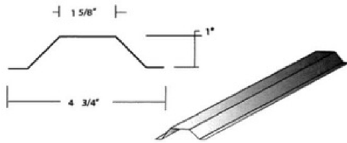
1" Sub-Girt
