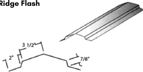
Ridge Flash
