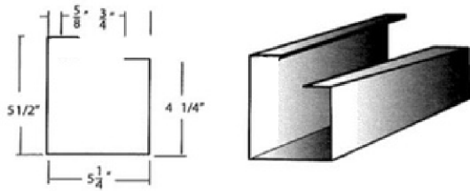
Straight Downspout
