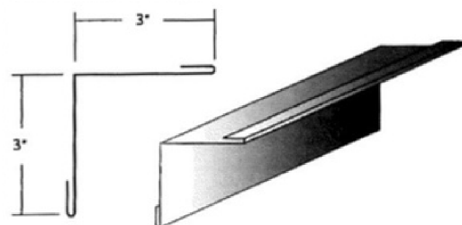
3 x 3 Inside Angle
