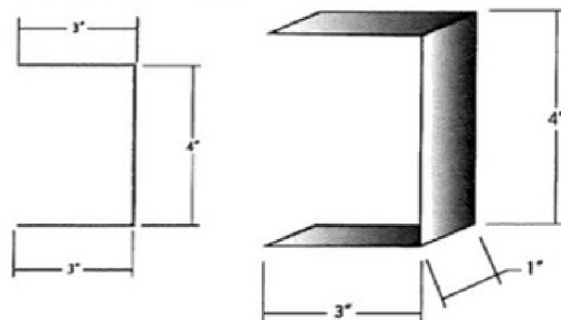
Downspout Strap
