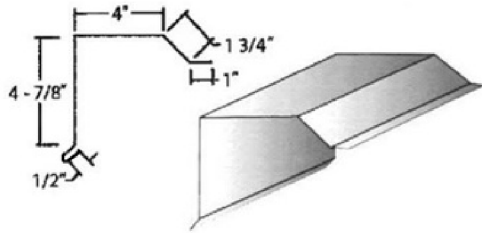
Rake Trim
